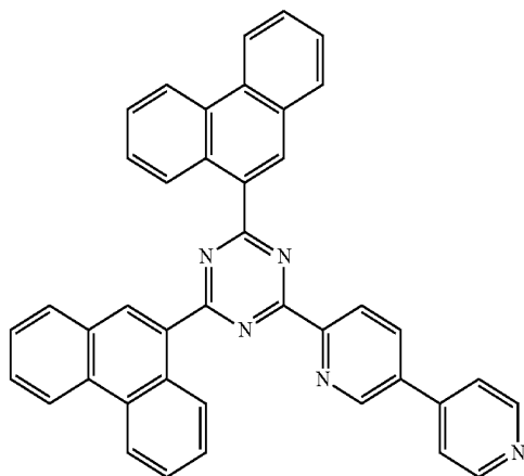
[Chemical Formula A-14]
