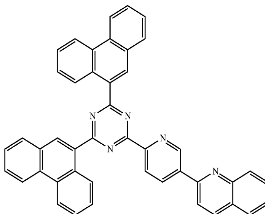
[Chemical Formula A-35]
