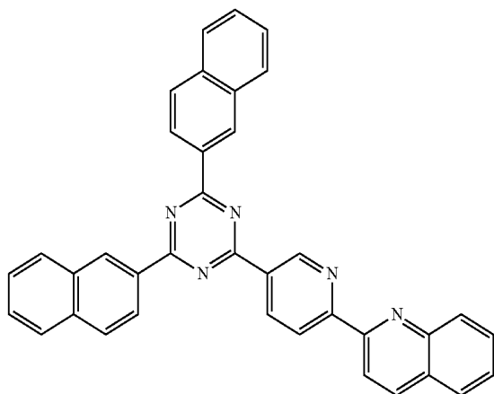
[Chemical Formula A-30]
