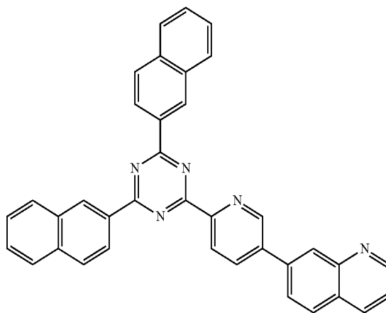
[Chemical Formula A-39]
