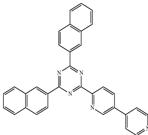
[Chemical Formula A-15]
