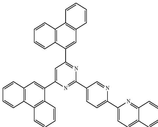
[Chemical Formula A-28]
