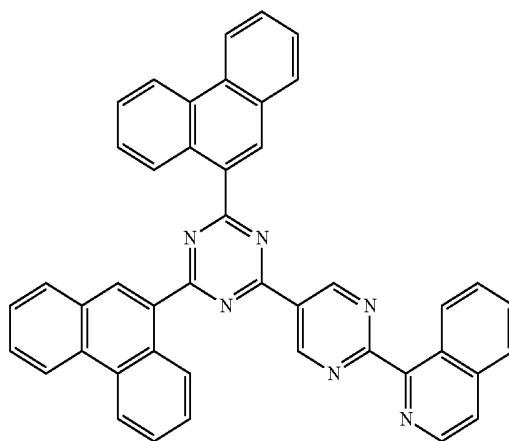
[Chemical Formula A-47]
