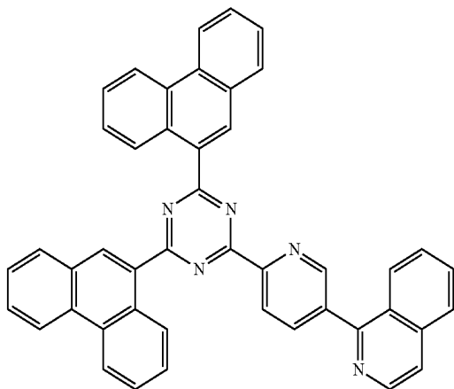
[Chemical Formula A-26]
