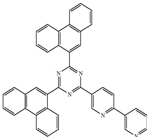
[Chemical Formula A-2]
