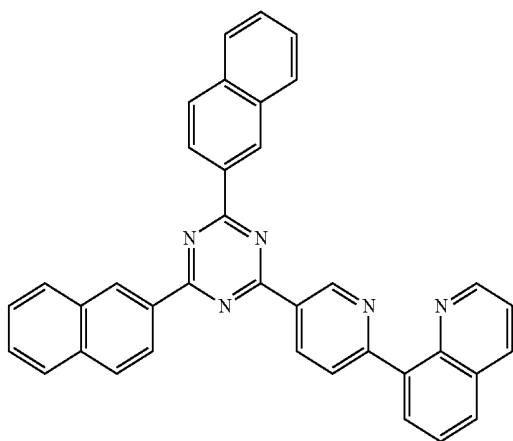
[Chemical Formula A-6]
