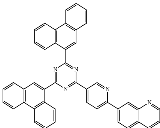
[Chemical Formula A-32]
