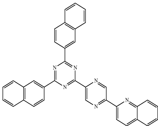
[Chemical Formula A-42]
