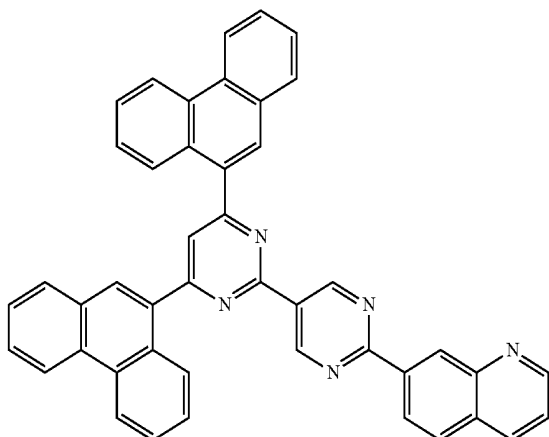
[Chemical Formula A-49]
