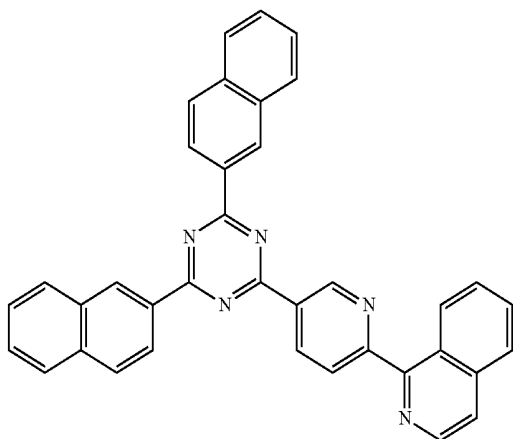
[Chemical Formula A-24]
