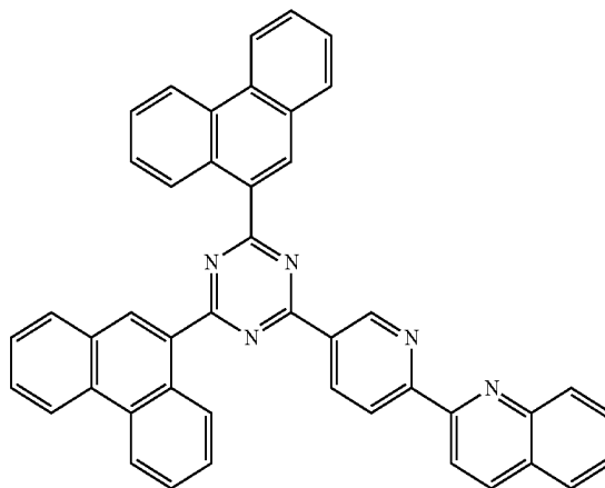
[Chemical Formula A-29]
