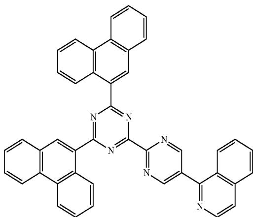
[Chemical Formula A-44]
