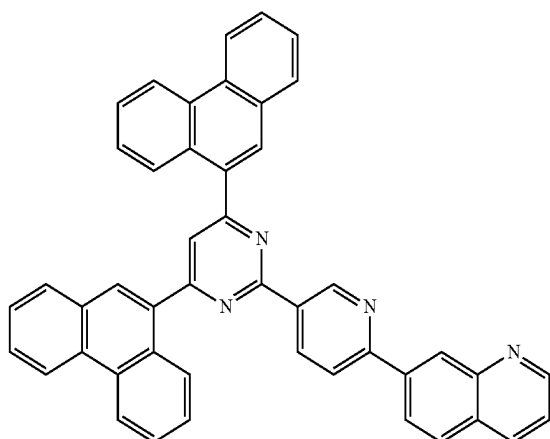
[Chemical Formula A-31]
