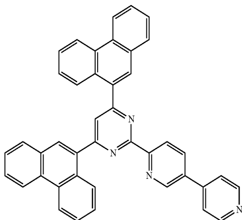
[Chemical Formula A-13]
