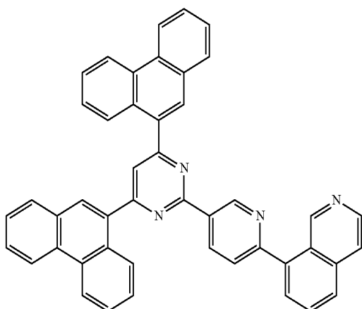
[Chemical Formula A-19]
