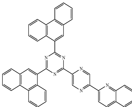
[Chemical Formula A-41]
