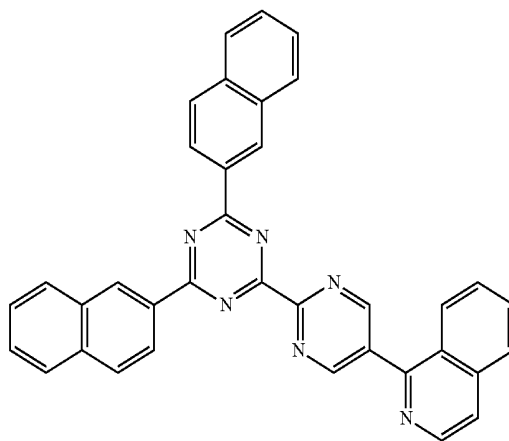
[Chemical Formula A-45]
