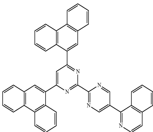
[Chemical Formula A-43]
