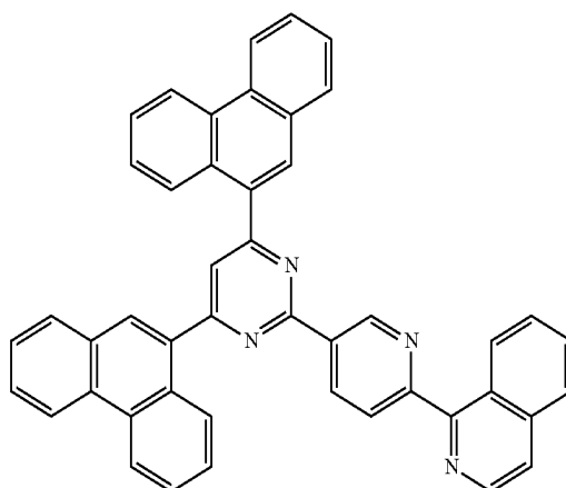
[Chemical Formula A-22]
