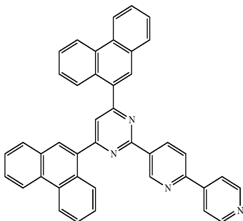
[Chemical Formula A-7]
