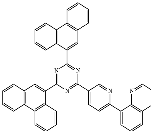
[Chemical Formula A-5]
