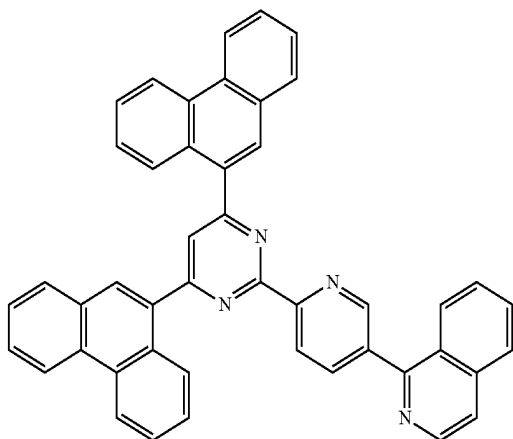
[Chemical Formula A-25]
