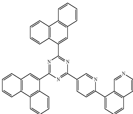
[Chemical Formula A-20]
