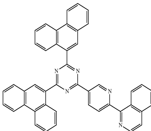
[Chemical Formula A-23]
