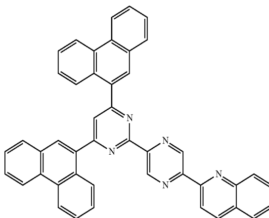
[Chemical Formula A-40]
