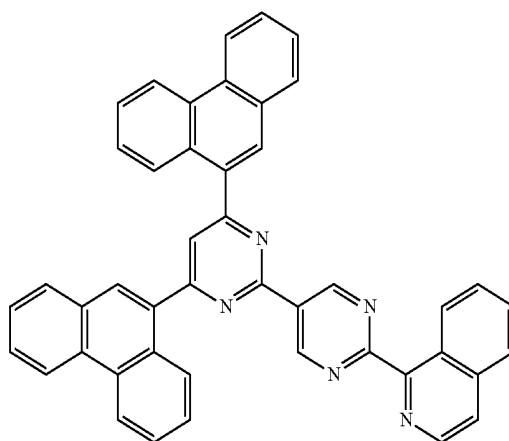
[Chemical Formula A-46]
