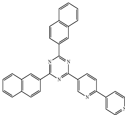
[Chemical Formula A-9]
