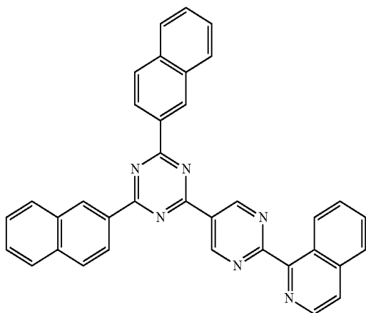
[Chemical Formula A-48]
