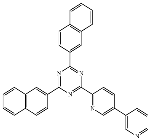
[Chemical Formula A-12]
