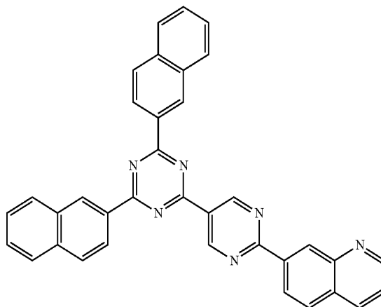
[Chemical Formula A-51]
