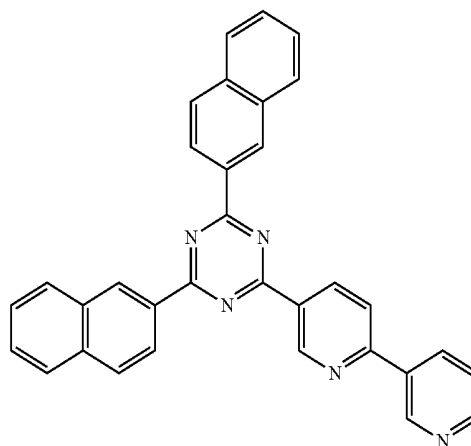
[Chemical Formula A-3]
