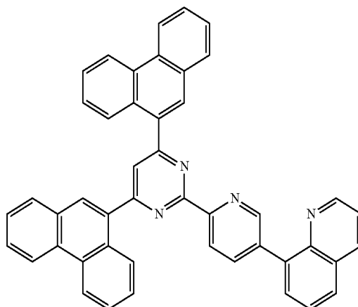
[Chemical Formula A-16]
