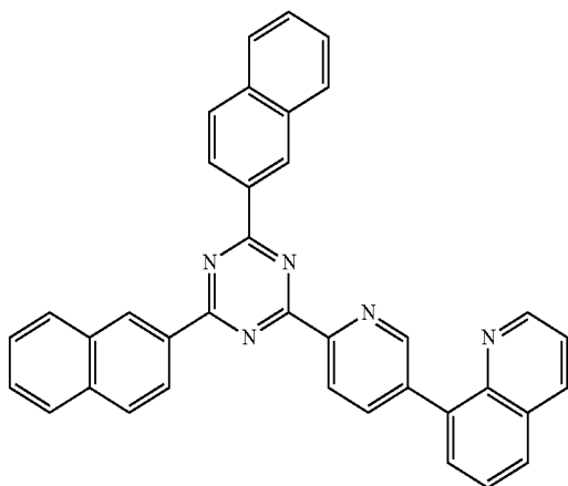
[Chemical Formula A-18]
