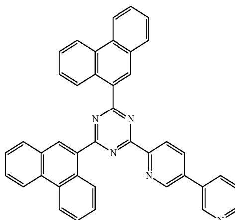
[Chemical Formula A-11]
