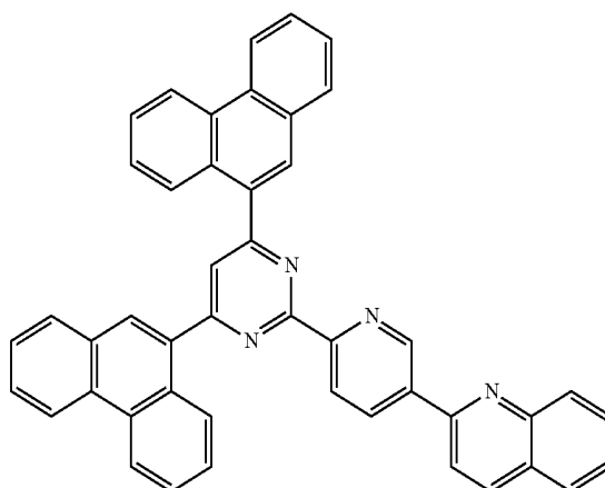
[Chemical Formula A-34]
