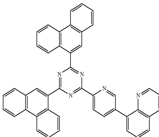
[Chemical Formula A-17]
