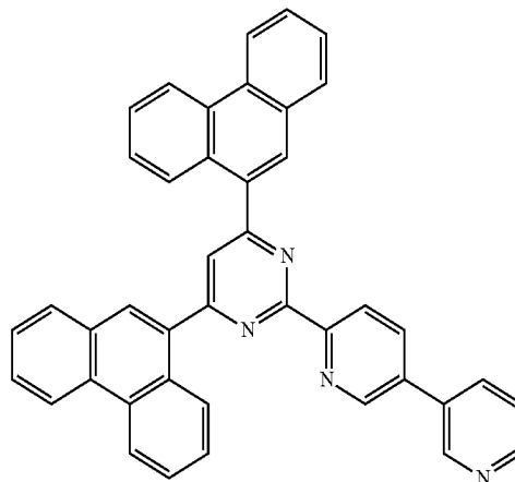
[Chemical Formula A-10]
