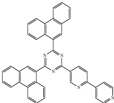
[Chemical Formula A-8]
