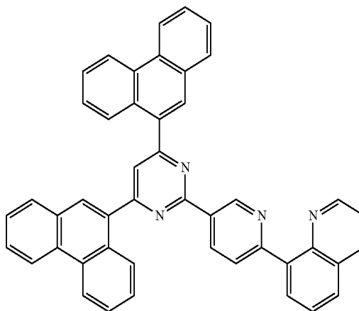
[Chemical Formula A-4]
